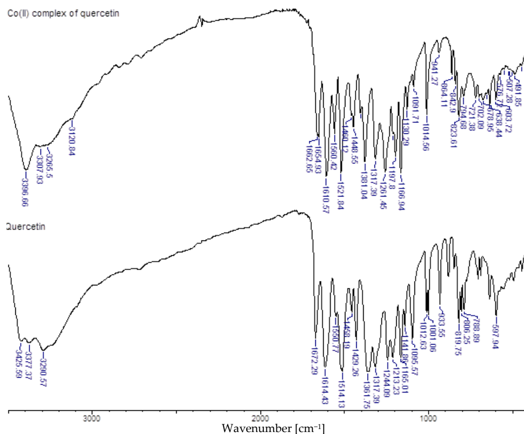
Figure 2. The FT-IR spectra of Co(II) complex of quercetin and quercetin registered in the range 4000–400 \text{cm}^{-1} .
