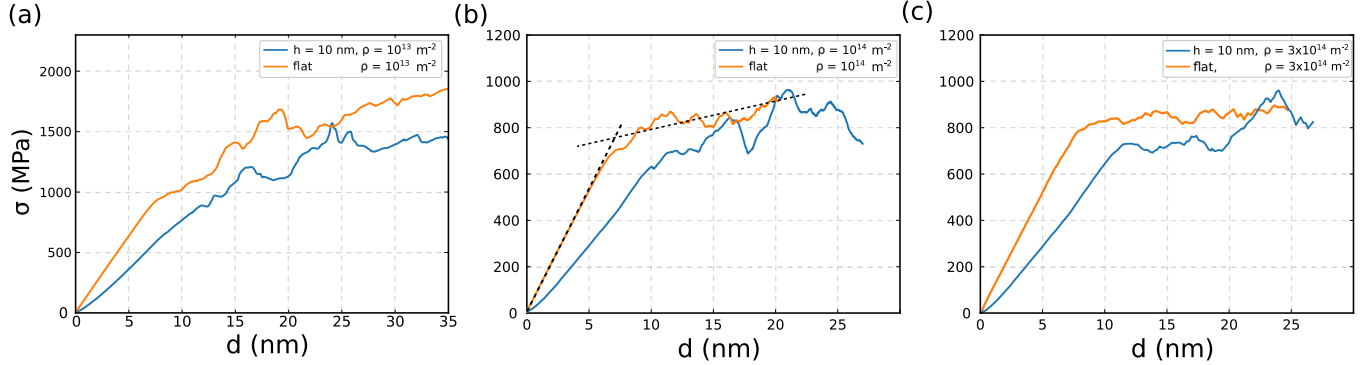
Fig. 5. (Color online) Stress–displacement curve obtained from the simulation of a flat pillar and a pillar with h = 10 \text{ nm} and initial dislocation density \rho = 10^{13} \text{ m}^{-2} (a), \rho = 10^{14} \text{ m}^{-2} (b) and \rho = 3 \times 10^{14} \text{ m}^{-2} (c).
