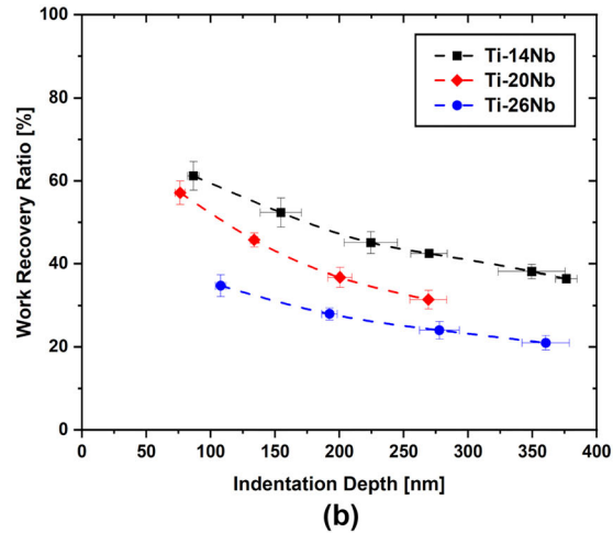
Fig. 8—Depth recovery ratio (a) and work recovery ratio (b) with respect to indentation depth for the investigated materials.
