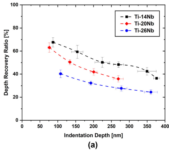
Fig. 8—Depth recovery ratio (a) and work recovery ratio (b) with respect to indentation depth for the investigated materials.
