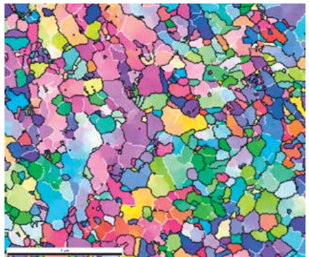
Fig. 3. EBSD orientation imaging microscopy map of HEA obtained in transmission mode (Transmission Kikuchi Diffraction - TKD).
