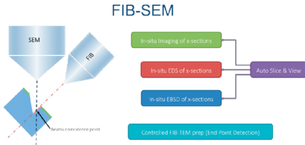
Fig. 2. Schematic representation of the dual-beam concept (FIB-SEM)
