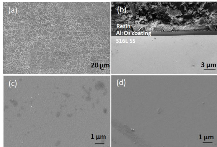
Fig. 2. SEM images of: (a) etched 316L SS surface; as-deposited PLD-grown Al 2 O 3 coating on 316L SS: (b) cross-section, (c) surface; (d) surface of PLD-grown Al 2 O 3 coating after ion-irradiation (50 dpa).
