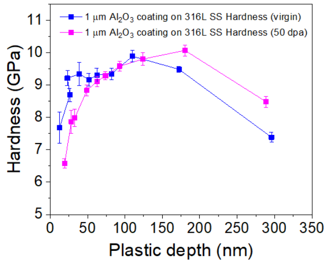
Fig. 6. Nanohardness of virgin and irradiated up to 50 dpa 1 \mu\text{m} \text{Al}_2\text{O}_3 coating on 316L SS plotted versus the plastic indentation depth.
